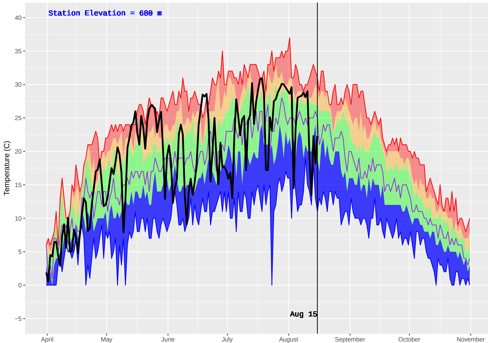
REVELSTOKE (363) : Historical (1995–2016) and Current (2018) Daily Temperature
