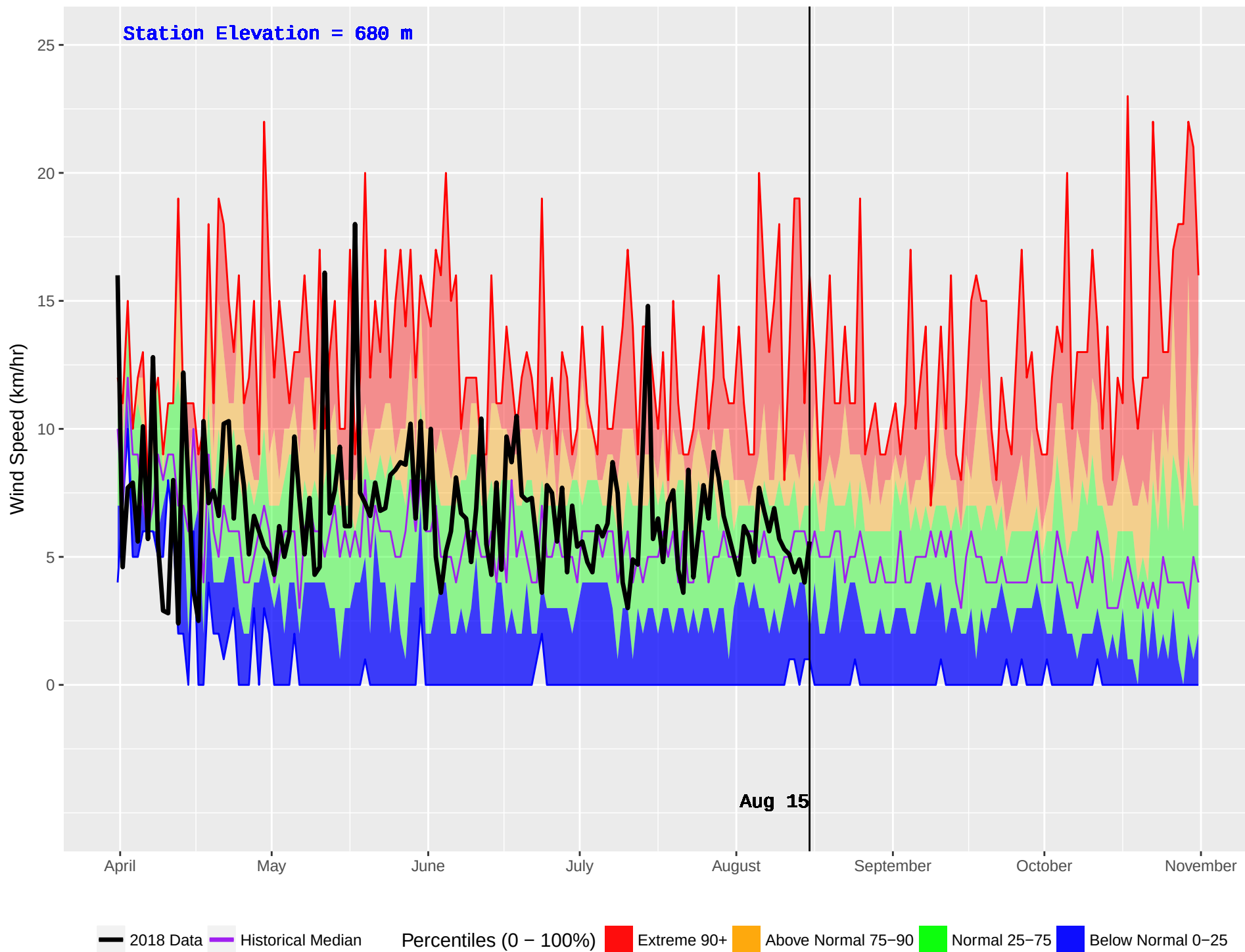
REVELSTOKE (363) : Historical (1995–2016) and Current (2018) Daily Wind Speed
