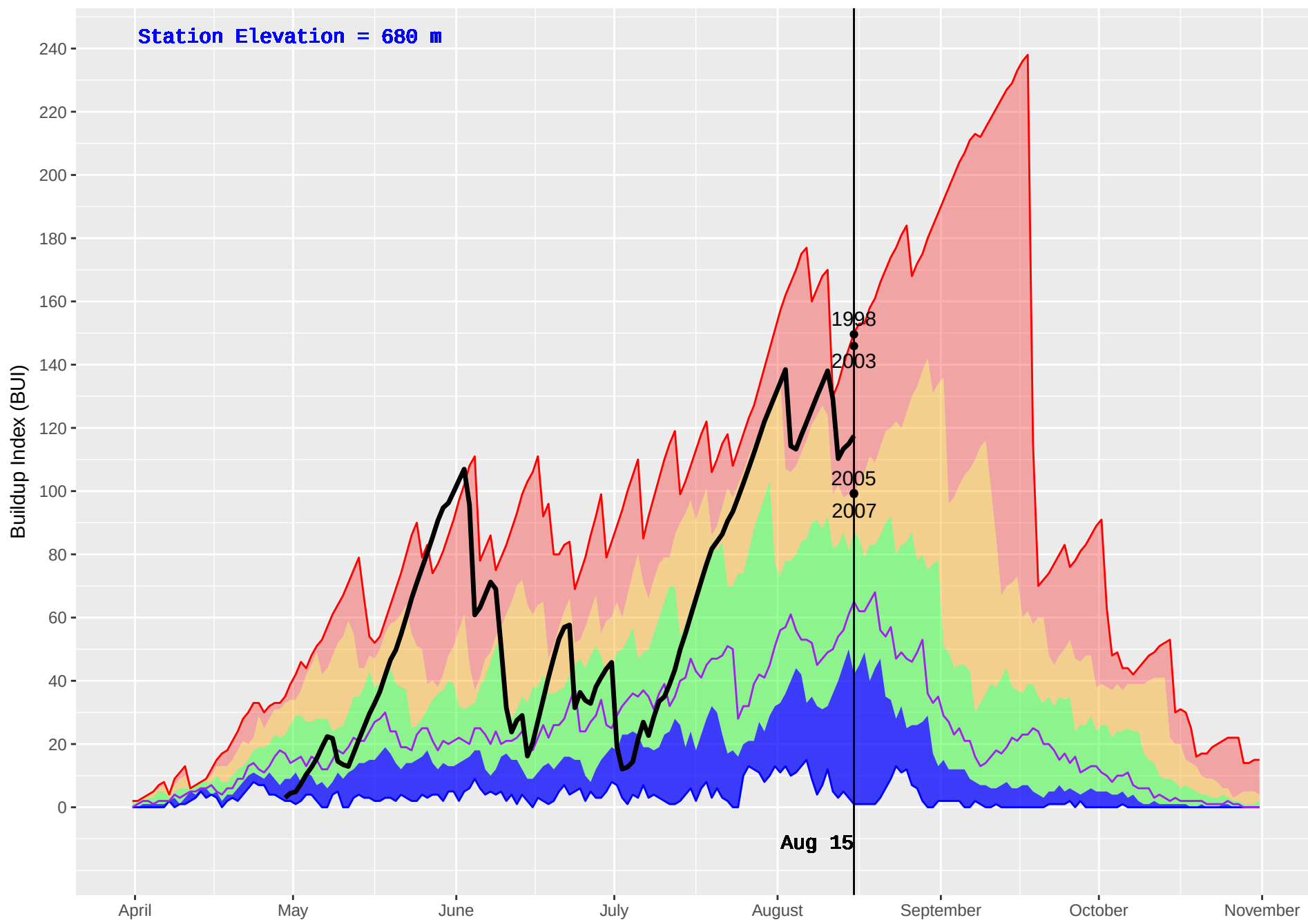
REVELSTOKE (363) : Historical (1995–2016) and Current (2018) Daily Buildup Index (BUI)
